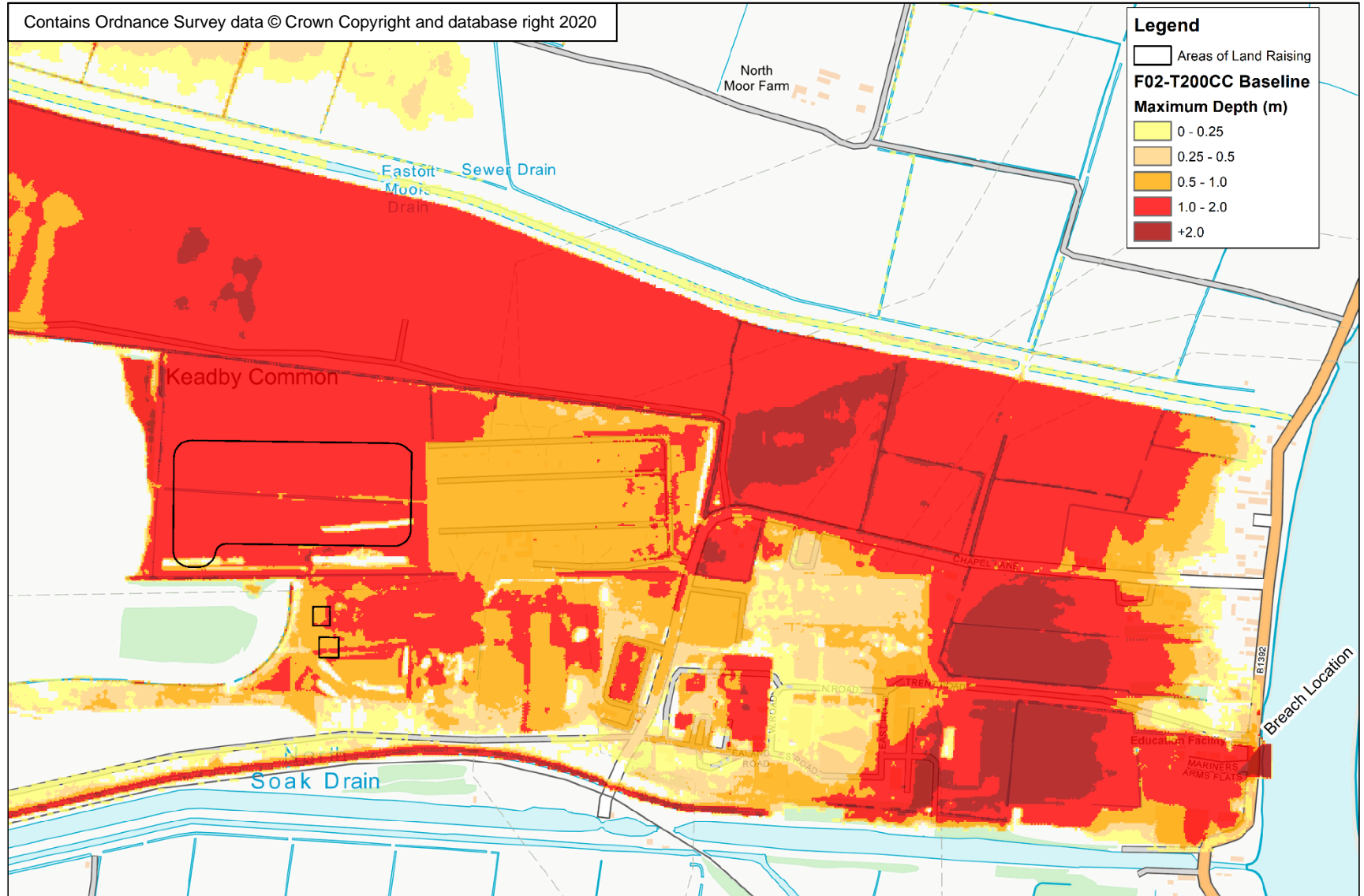
Figure 4-1 Maximum depth of inundation (defence breach, 200y tidal event with CC combined with 2y fluvial event) - Baseline
